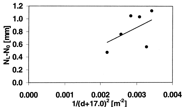
Fig. 3. BOL analysis of the 1997 Nieuwerkerk hoax with BOL at an (optimised) height of 17 m above the centre of the circular imprint. Straight line: least-squares best fit. Pearson coefficient: R = 0.54 .
