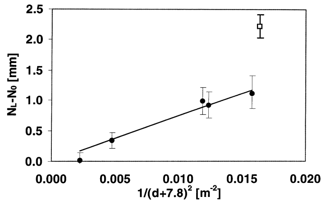
Fig. 2. BOL analysis of the 1994 Sussex formation. The BOL was set at a height of 7.8 m above the centre of the circular imprint. Straight line: least-squares best fit. Pearson coefficient: R = 0.97 .
